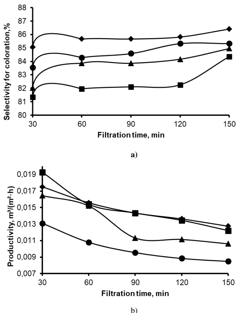
Figure 5 – Effect of PVA dosage on a) selectivity for coloration; b) productivity of the filtration material: ■ – 10%, ♦ – 20%, ▲ – 30%, ● – 40%.
