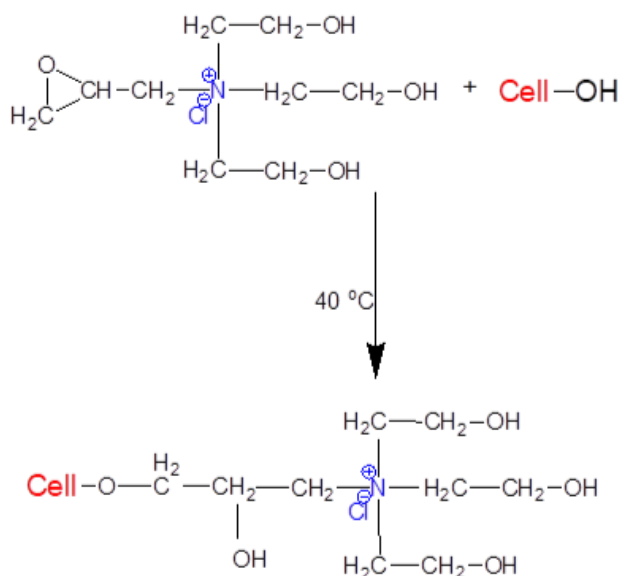
Fig.2. Reaction of cellulose with the aminating mixture
